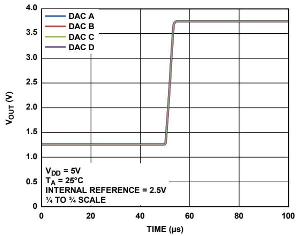
Figure 31. Settling Time
