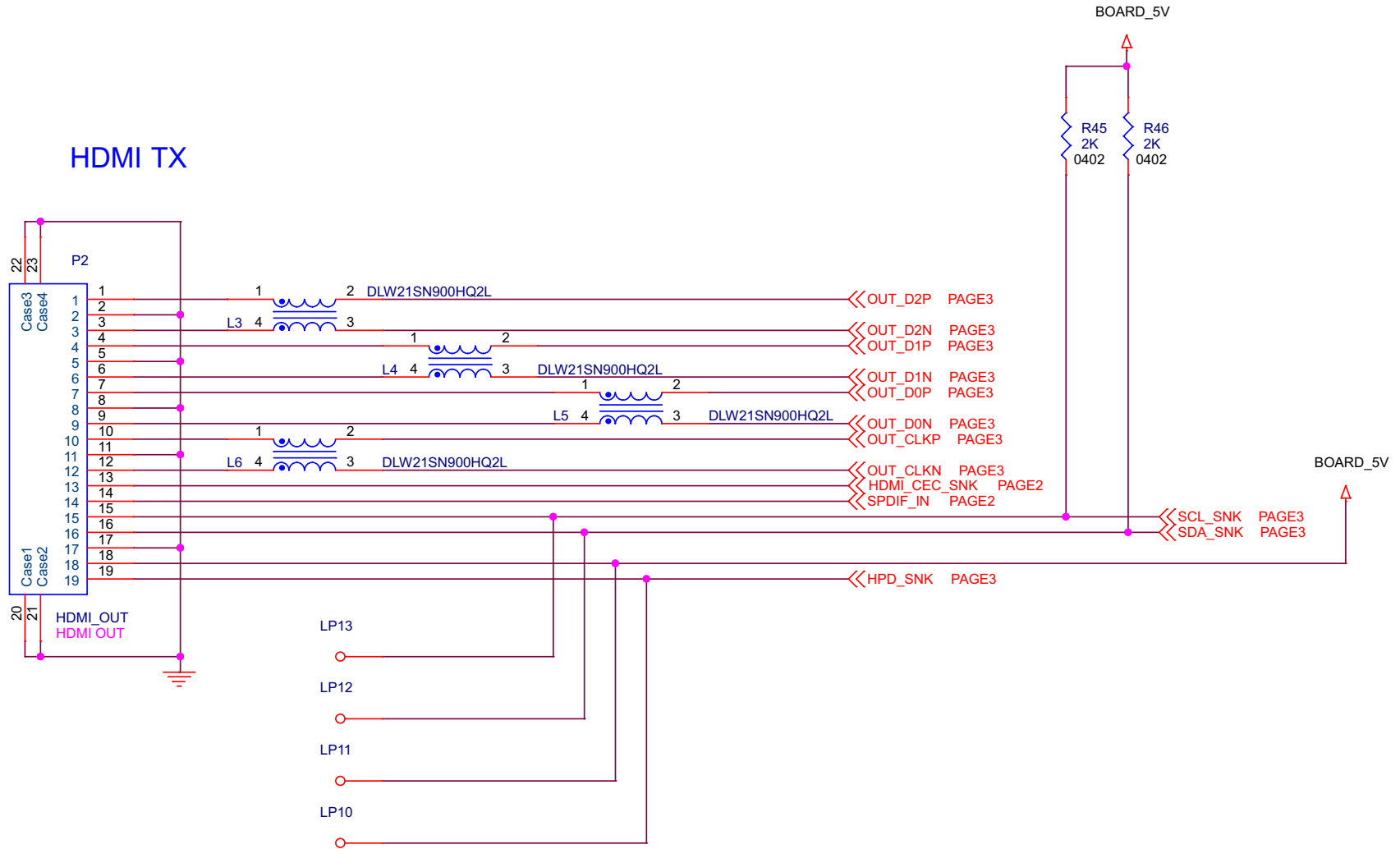
Figure 7. DP149RSBEVM HDMI Schematic
