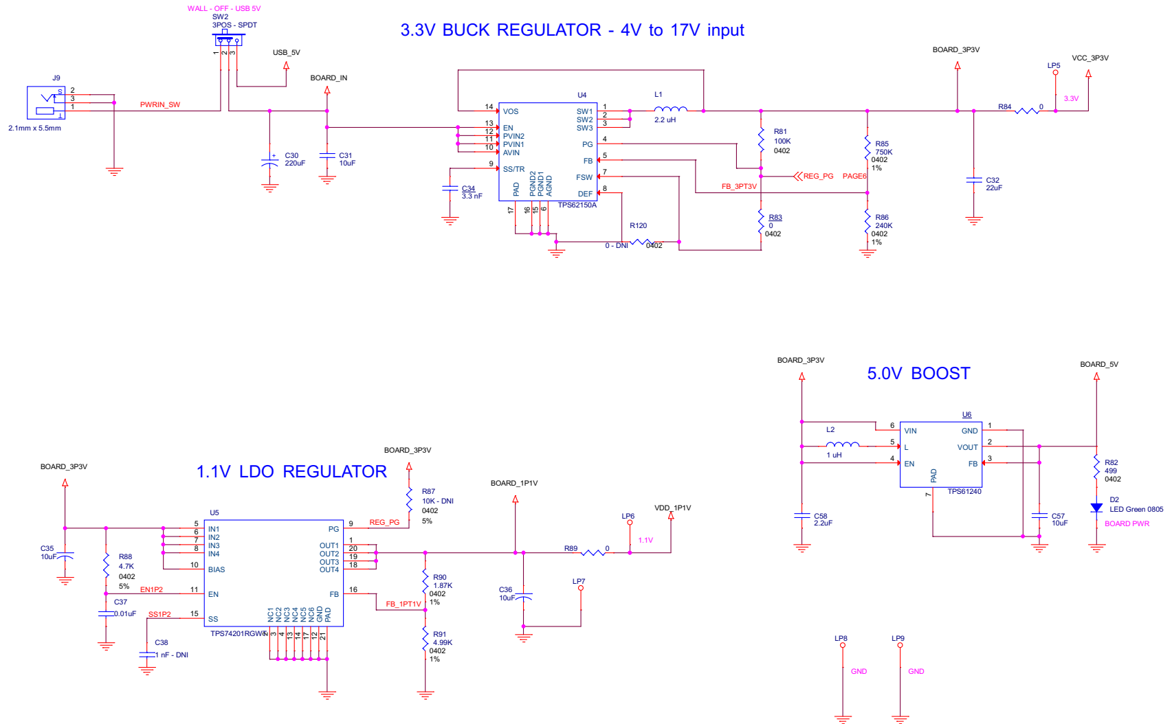
Figure 10. DP149RSBEVM Regulators Schematic
