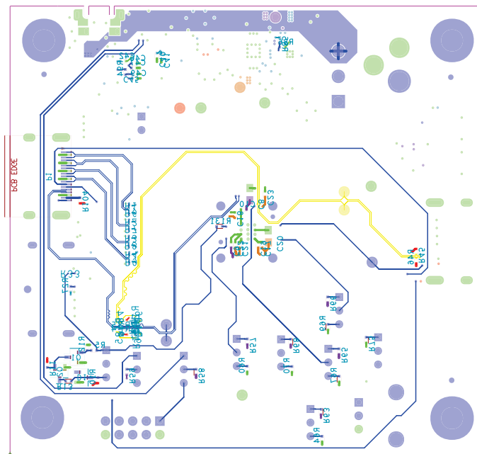
Figure 17. Layer 6 (Bottom)
