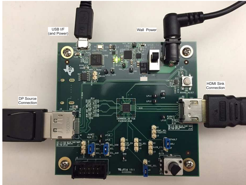
Figure 1. DP149RSBEVM
