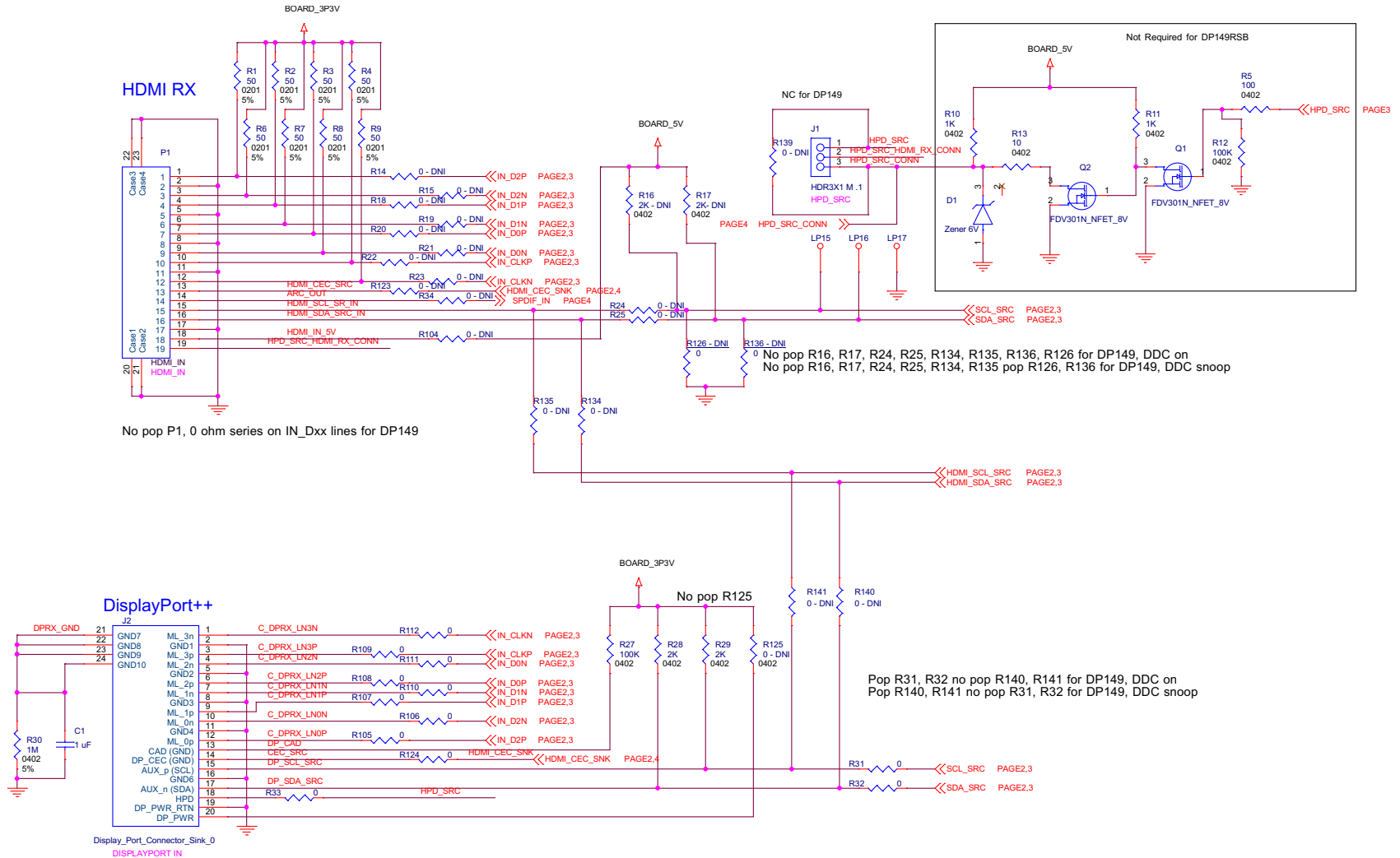
Figure 5. DP149RSBEVM Input Connectors Schematic
