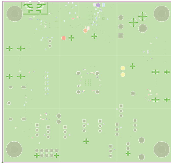
Figure 16. Layer 5 (GND)
