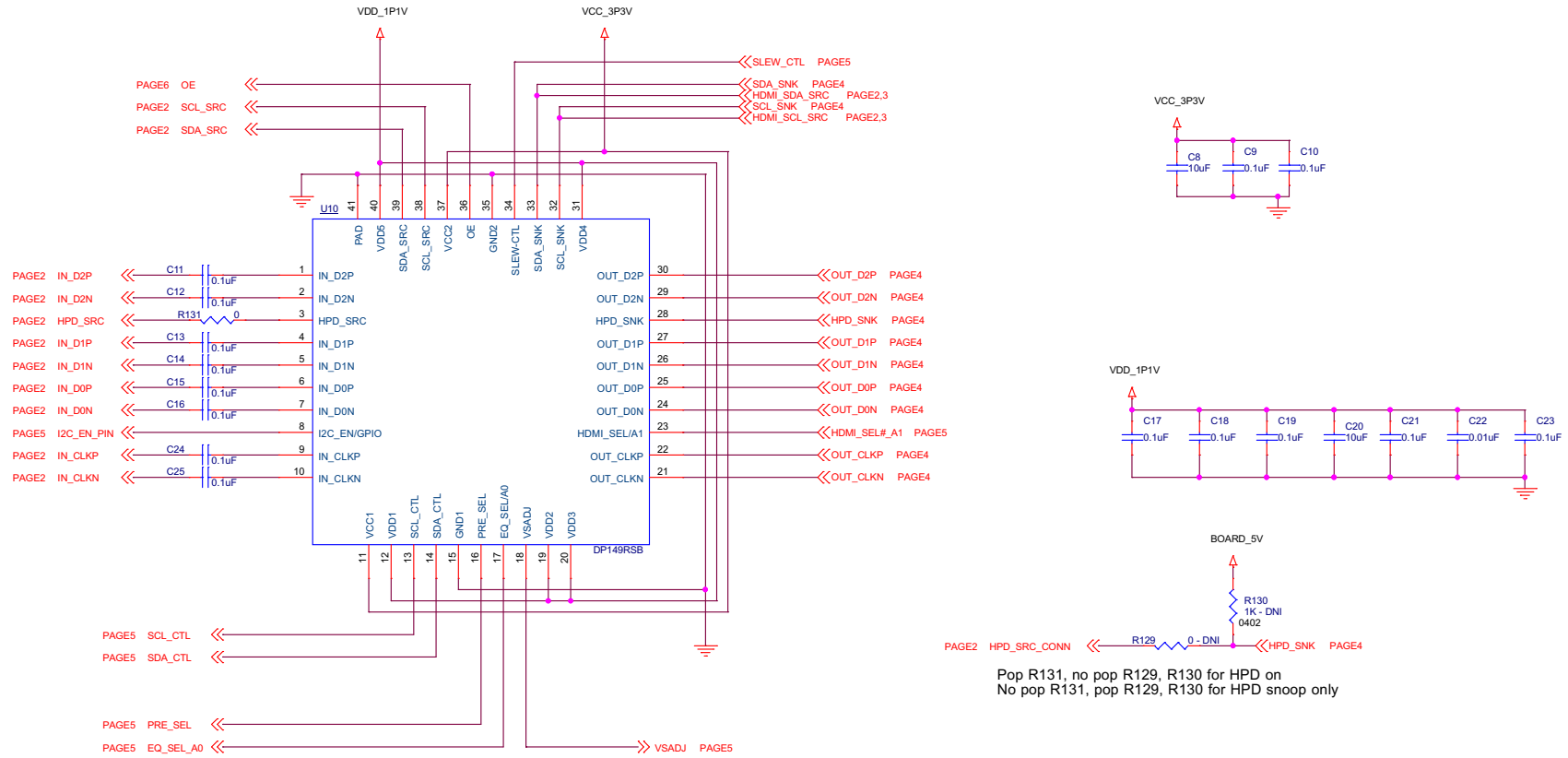
Figure 6. DP149RSB Schematic
