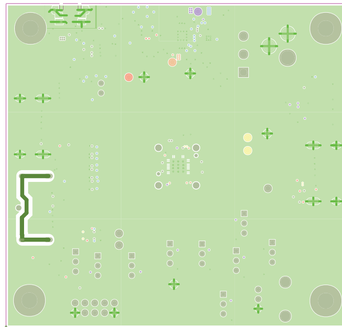
Figure 13. Layer 2 (GND)
