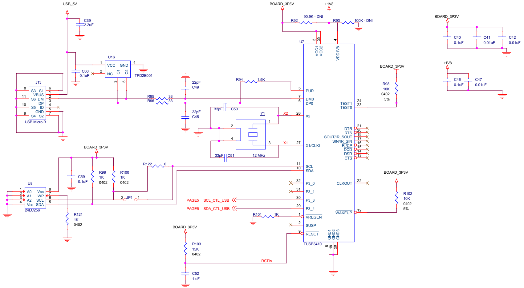
Figure 11. DP149RSBEVM TUSB3410 Schematic
