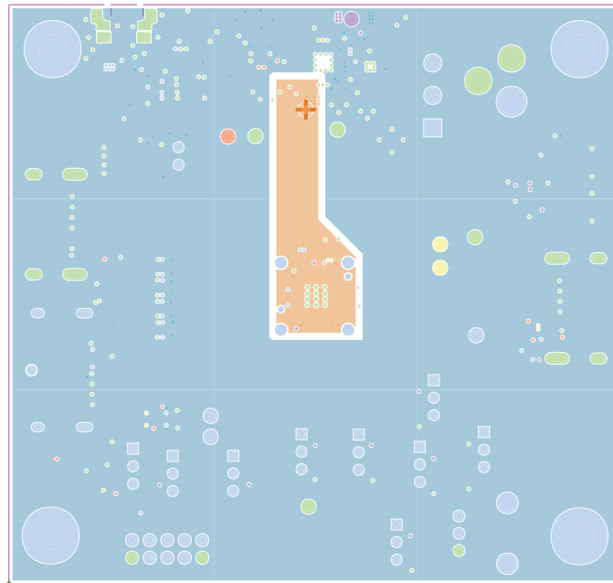
Figure 14. Layer 3 (Power)
