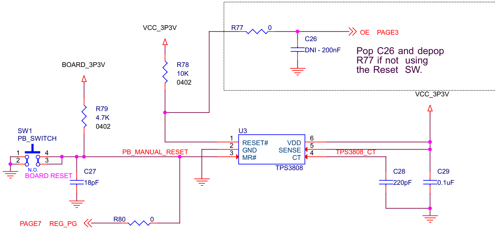
Figure 9. DP149RSBEVM Reset Schematic
