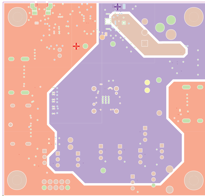
Figure 15. Layer 4 (Power)
