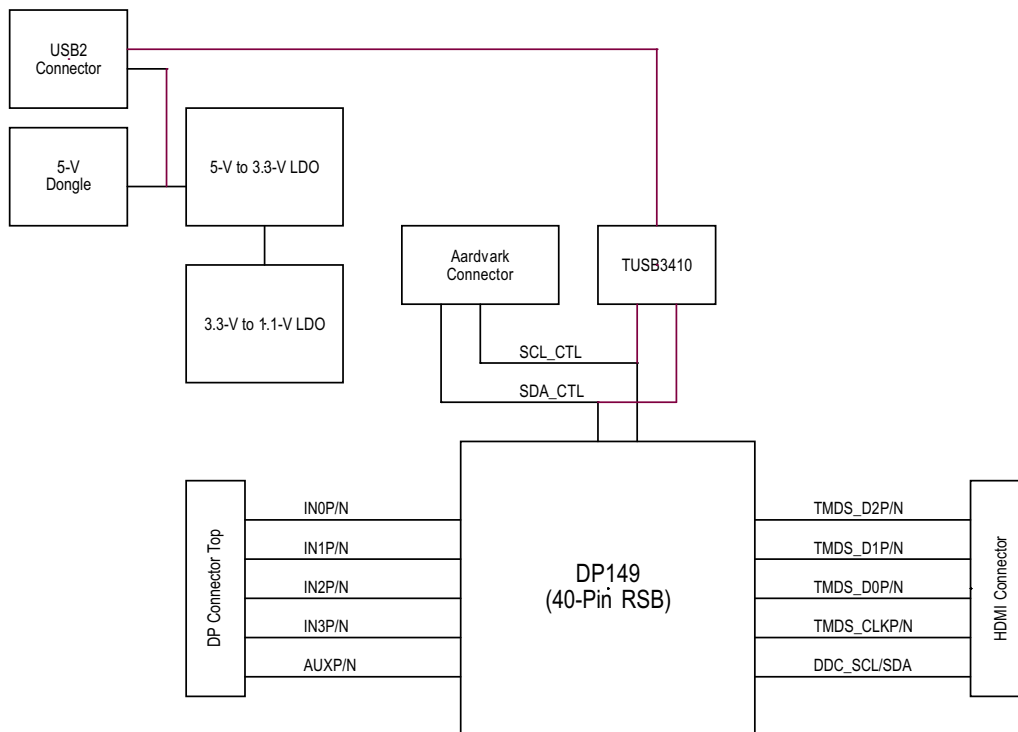
Figure 2. DP149RSB EVM Block Diagram
