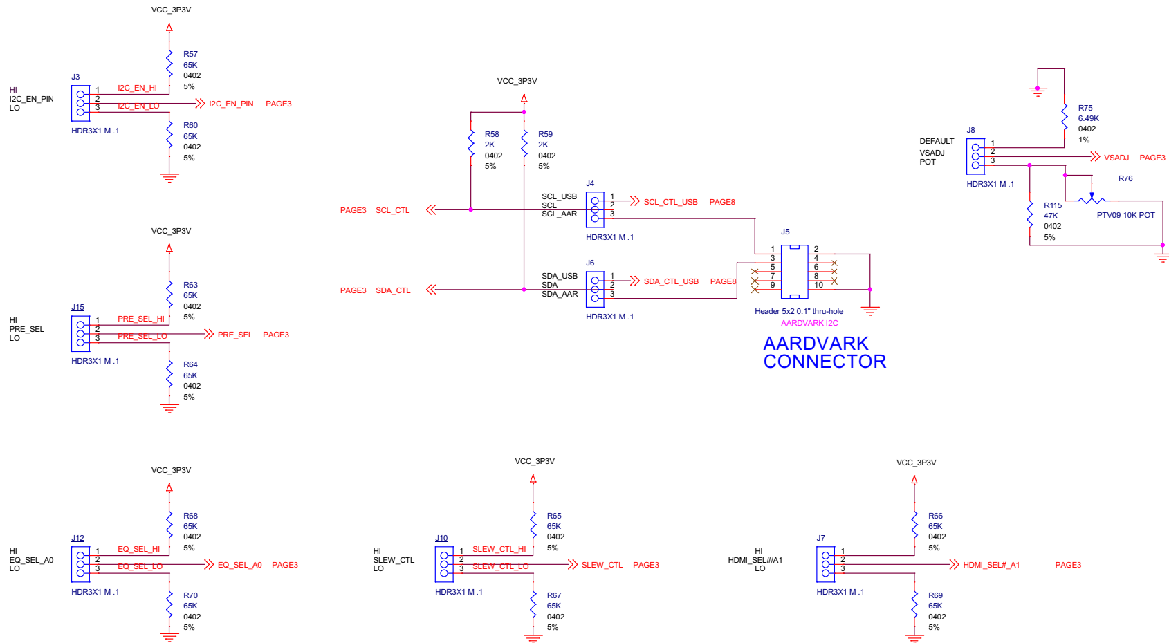
Figure 8. DP149RSBEVM Select Options Schematic
