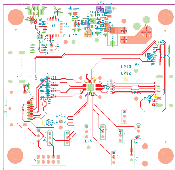
Figure 12. Layer 1 (Top)
