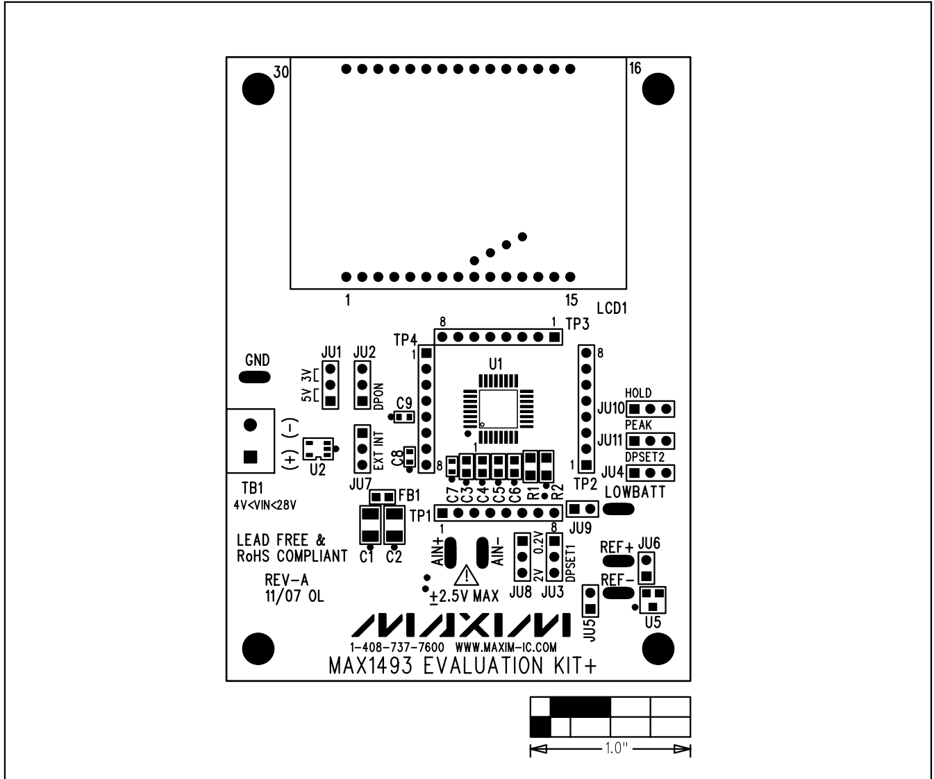
Figure 2. MAX1493 EV Kit Component Placement Guide—Component Side
