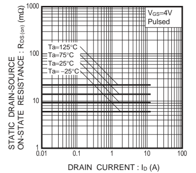
Fig.9 Static Drain-Source On-State Resistance vs. Drain Current (III)
