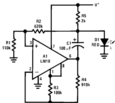
Figure 61. Battery-level Indicator
