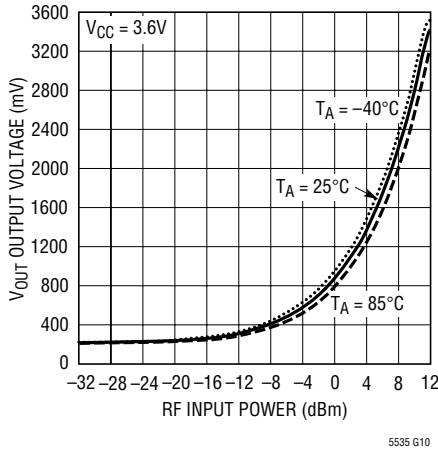
V_{OUT} vs RF Input Power and V_{OS} , 2000MHz, Gain = 2
