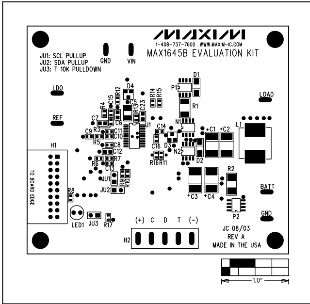
Figure 6. MAX1645B EV Kit Component Placement Guide—Component Side
