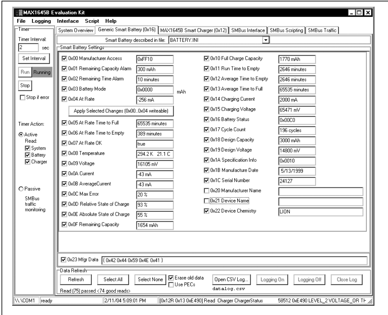
Figure 4. MAX1645B Smart-Battery Command Panel
