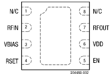
Figure 2. SKY67183-396LF Pinout (Top View)
