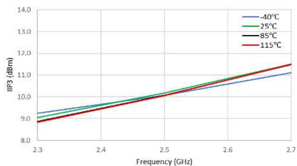
Figure 36. IIP3 (dBm) vs Frequency (GHz)
