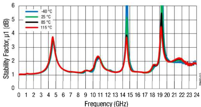
Figure 15. Stability Factor, \mu_1 (dB) vs Frequency (GHz)
