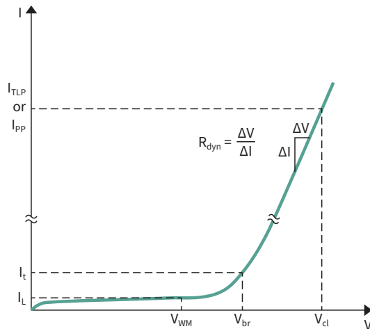
Fig. 3 Diode-like
