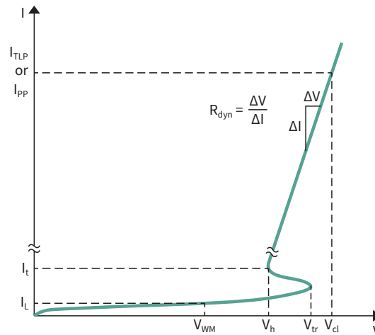
Fig. 4 Mild snapback
