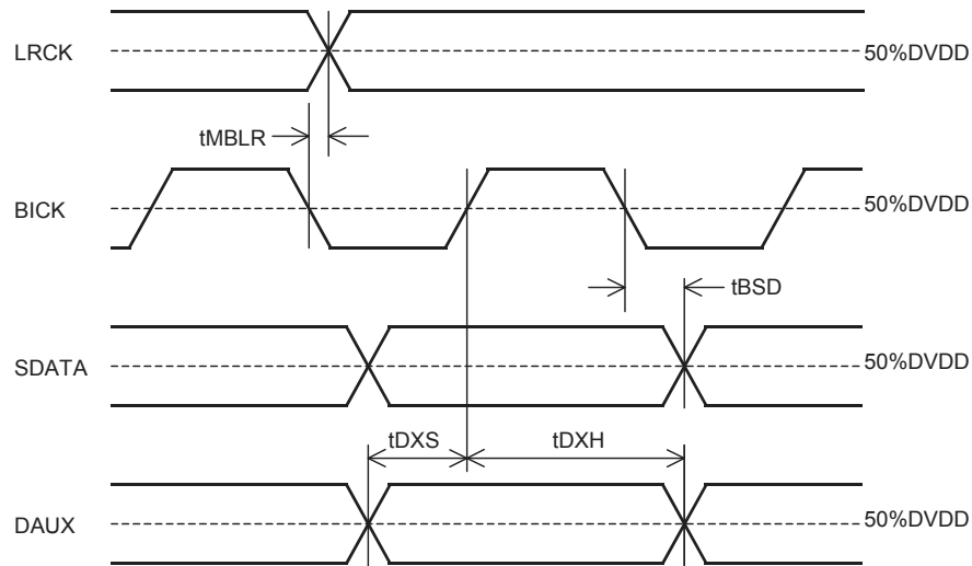
Serial Interface Timing (Master Mode)
