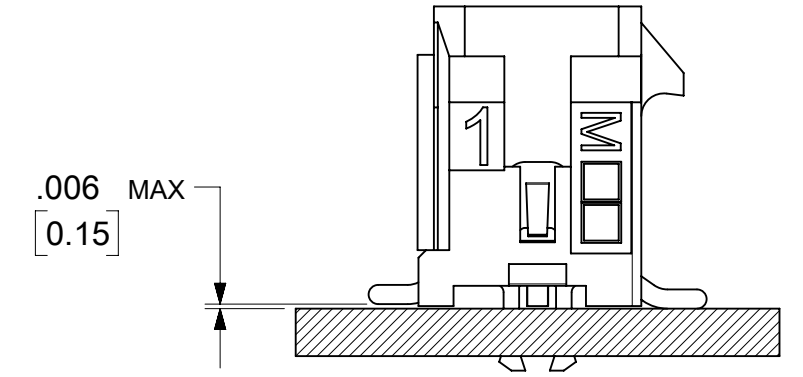
COPLANARITY DETAIL SEE NOTE #7
