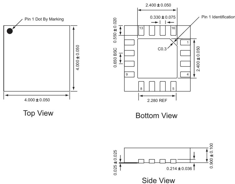
QFN44-16 3
