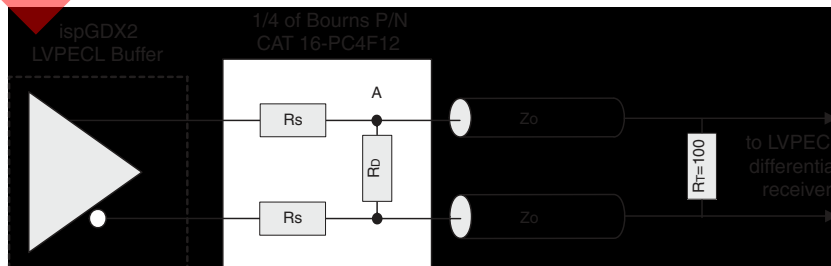
Figure 17. LVPECL Driver with Three Resistor Pack
