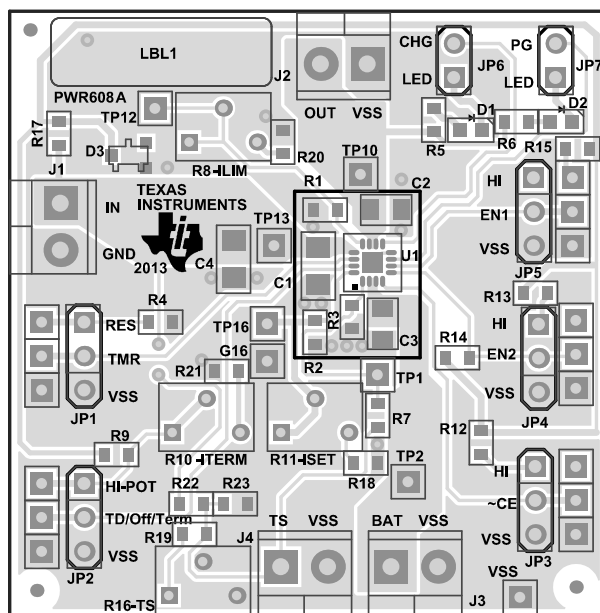
Figure 4. Top Assembly View
