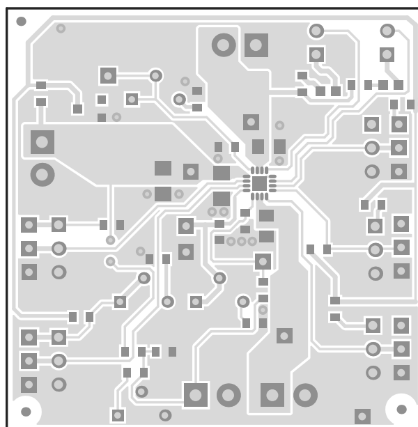
Figure 5. Board Layout – Top Etch Layer
