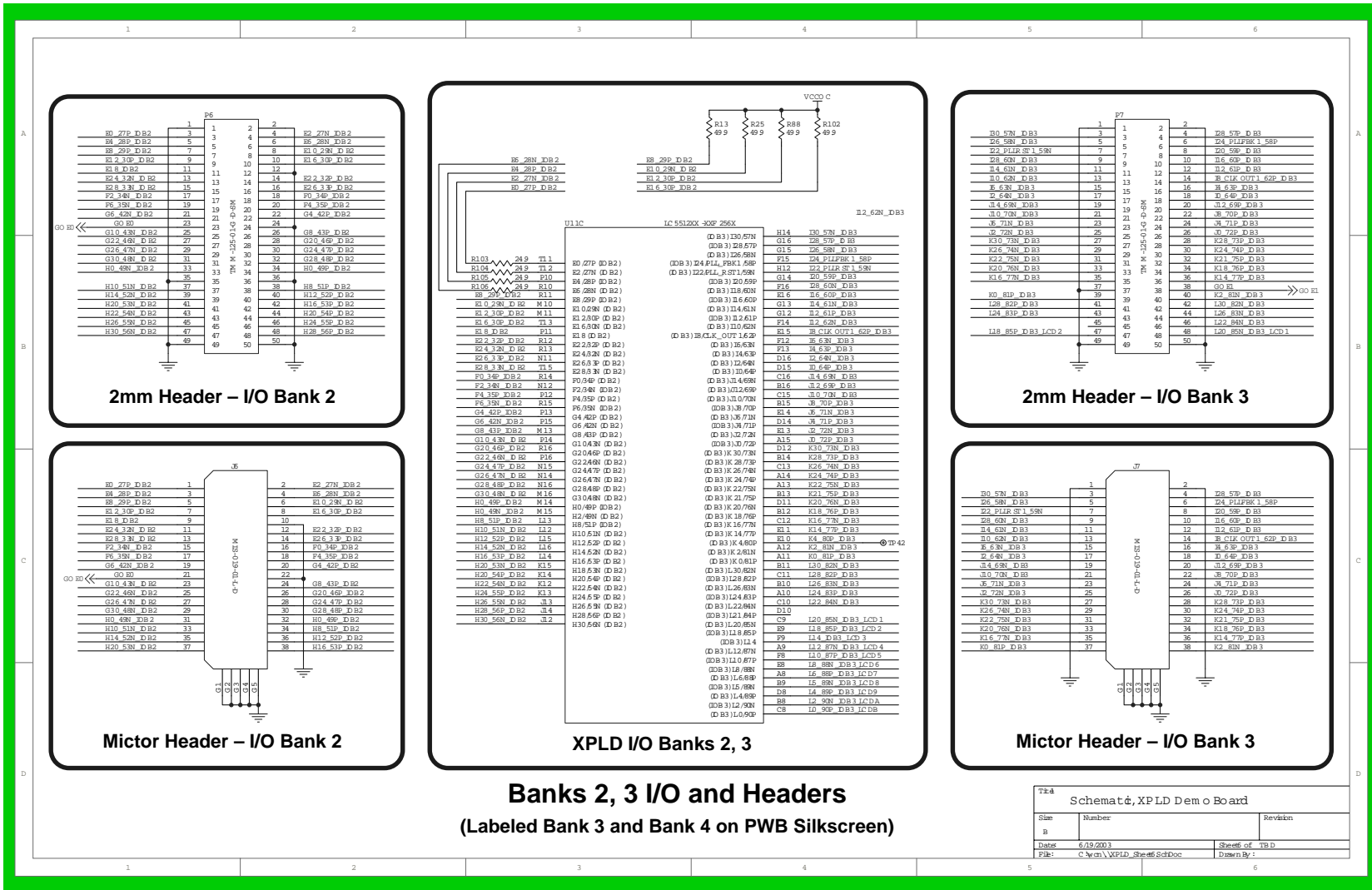
Figure 10. Lattice ispXPLD Evaluation Board Schematic
