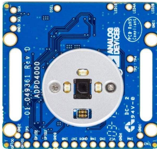
Figure 2. EVAL-ADPD4000Z-PPG Bottom Side, Optical
