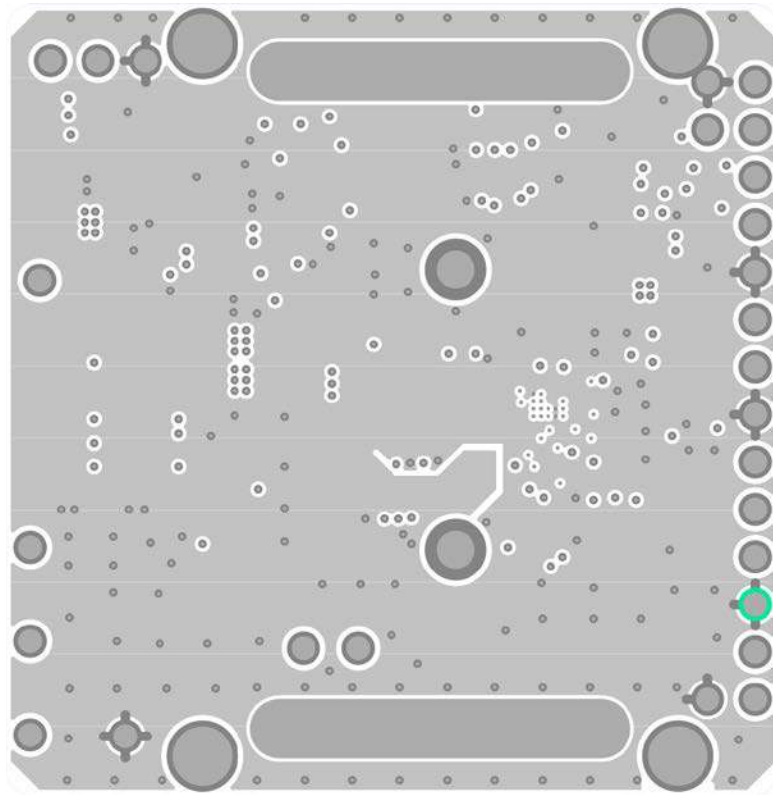
Figure 17. Layer 5, Ground
