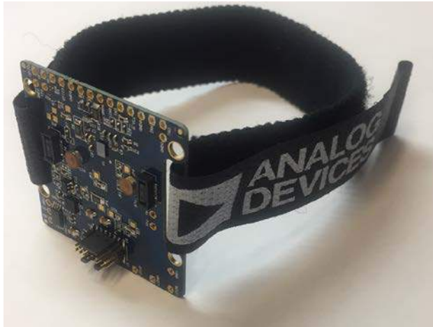
Figure 6. Optional Wrist Strap on EVAL-ADPD4000Z-PPG
