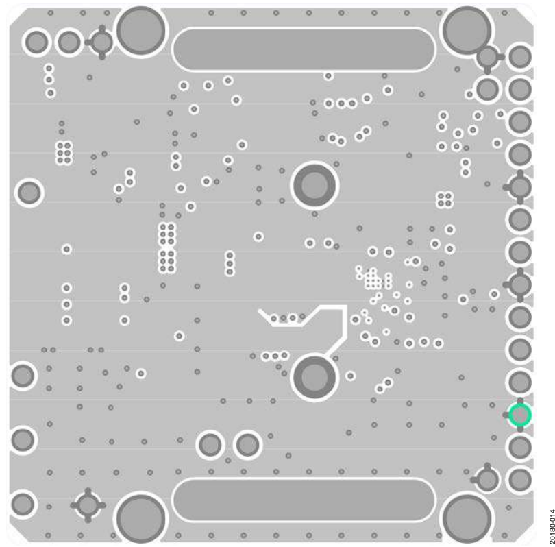
Figure 14. Layer 2, Ground
