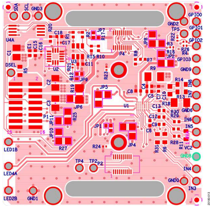
Figure 13. Component: Top Layer and Silkscreen
