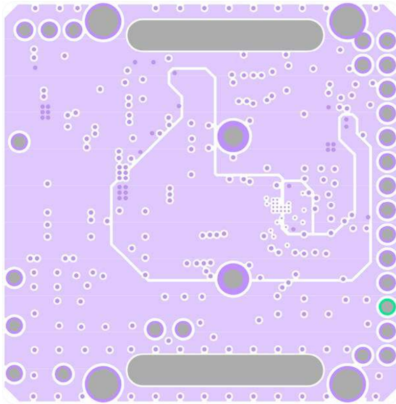
Figure 15. Layer 3, Power
