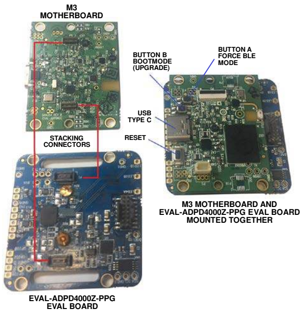
Figure 7. Connecting the EVAL-ADPDM3Z to the EVAL-ADPD4000Z-PPG
