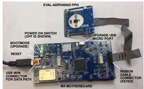
Figure 5. Connect the EVAL-ADPUCZ to the EVAL-ADPD4000Z-PPG
