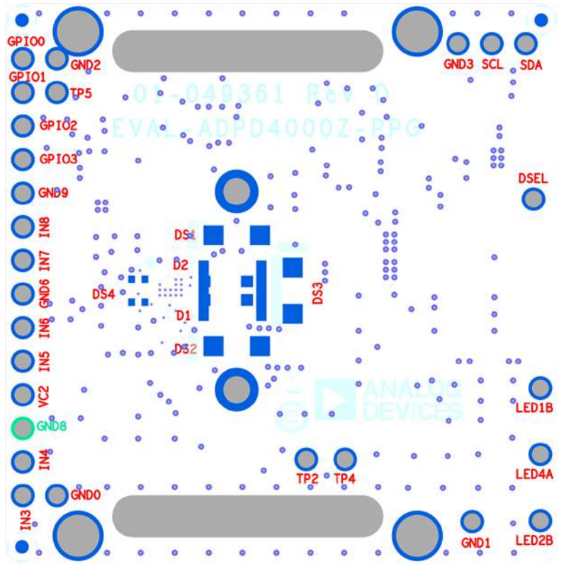
Figure 19. EVAL-ADPD4000Z-PPG Layout, Bottom Layer, Inverted Silkscreen View
