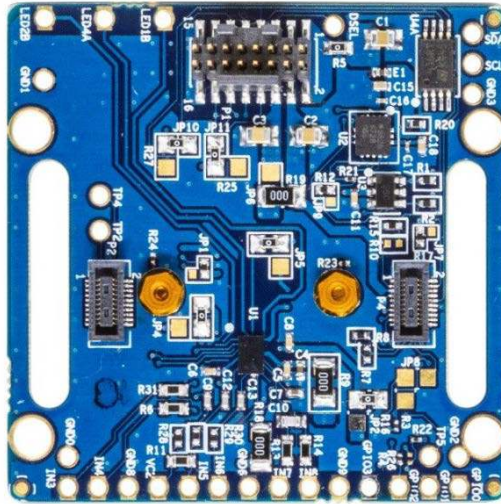
Figure 1. EVAL-ADPD4000Z-PPG Top Side
