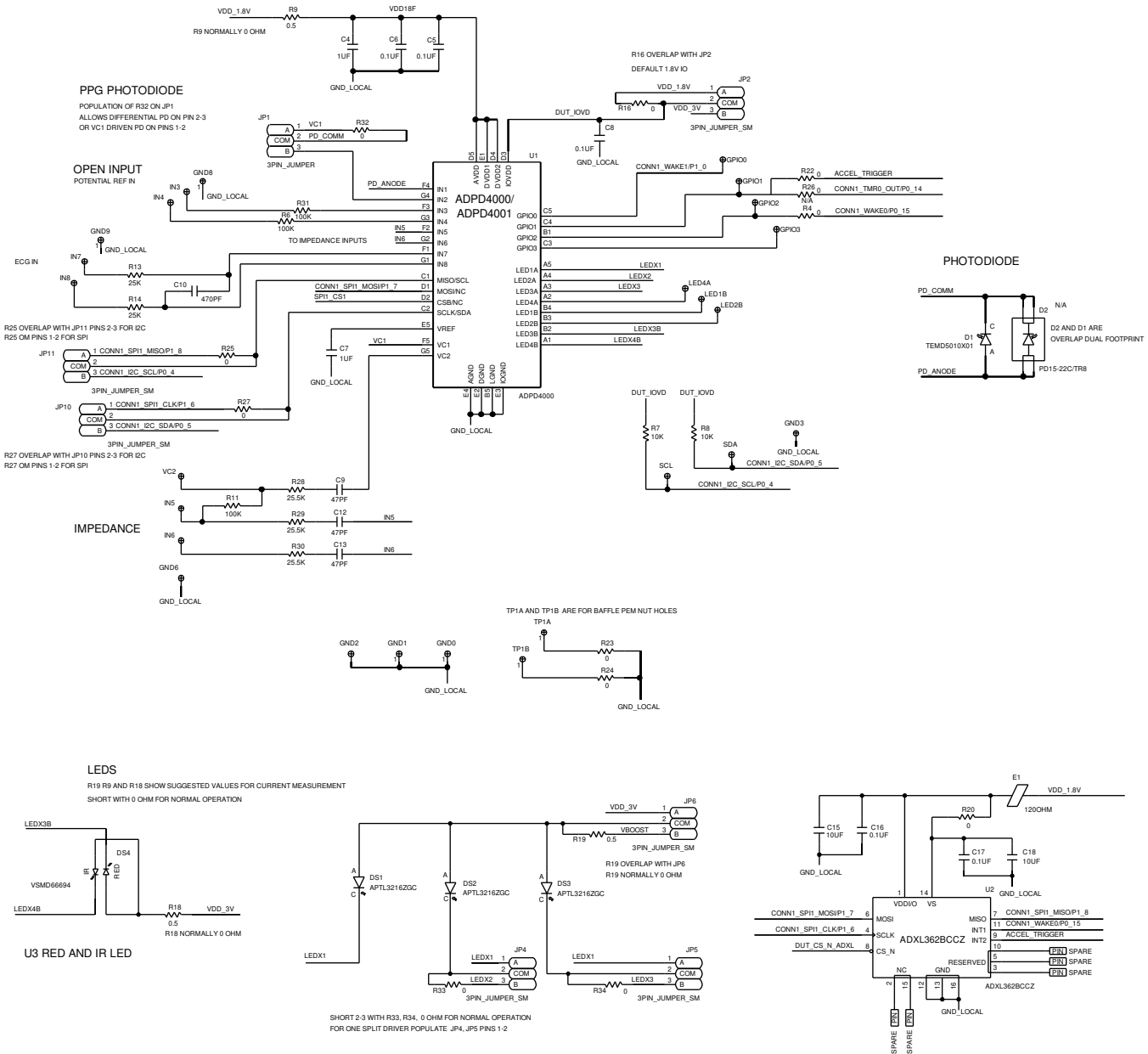
Figure 11. EVAL-ADPD400Z-PPG Schematic, Page 1
