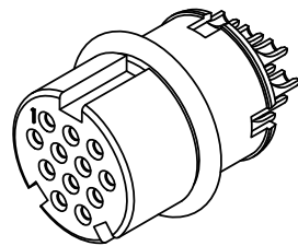
SF3282-10ESG-5XX FACE VIEW POS 11 & 12 MOLDED HALF CLOSED
