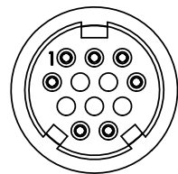
SF3282-7ESG-5XX FACE VIEW POS 5, 8, 10, 11 & 12 MOLDED HALF CLOSED
