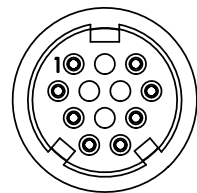
SF3282-8ESG-5XX FACE VIEW POS 2, 10, 11 & 12 MOLDED HALF CLOSED
