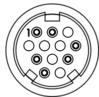
SF3282-6ESG-5XX FACE VIEW POS 3, 6, 9, 10, 11 & 12 MOLDED HALF CLOSED
