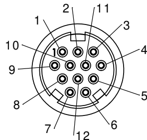
SF3282-12ESG-5XX FACE VIEW
