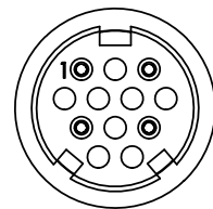
SF3282-4ESG-5XX FACE VIEW POS 2, 4, 6, 7, 9, 10, 11 & 12 MOLDED HALF CLOSED
