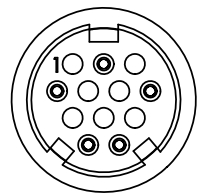
SF3282-5ESG-5XX FACE VIEW POS 1, 3, 5, 8, 10, 11 & 12 MOLDED HALF CLOSED
