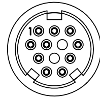
SF3282-10ESG-5XX FACE VIEW POS 11 & 12 MOLDED HALF CLOSED
