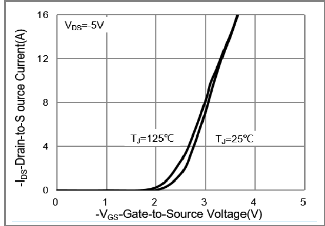
Fig.14 Transfer Characteristics
