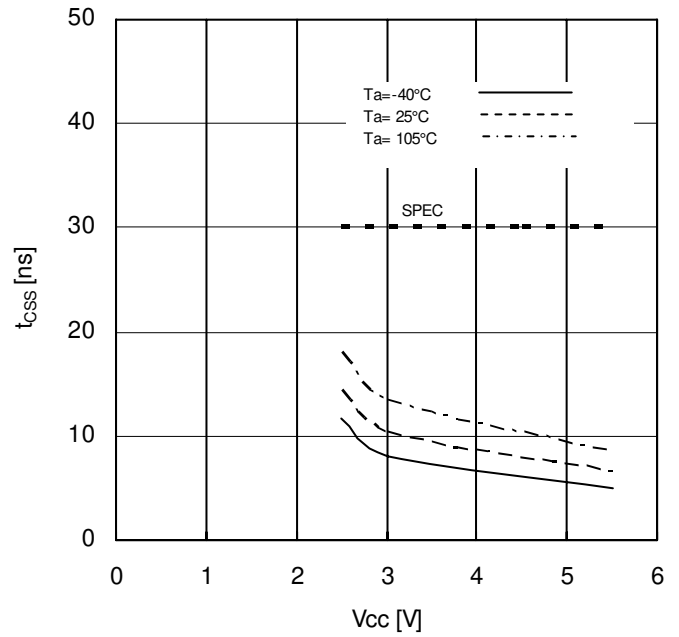
Figure 18. CSB Setup Time vs Supply Voltage
