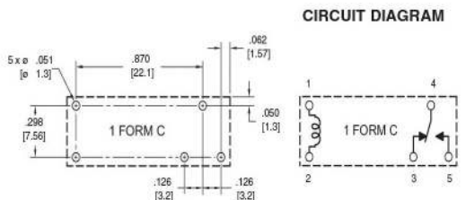
CIRCUIT DIAGRAM
