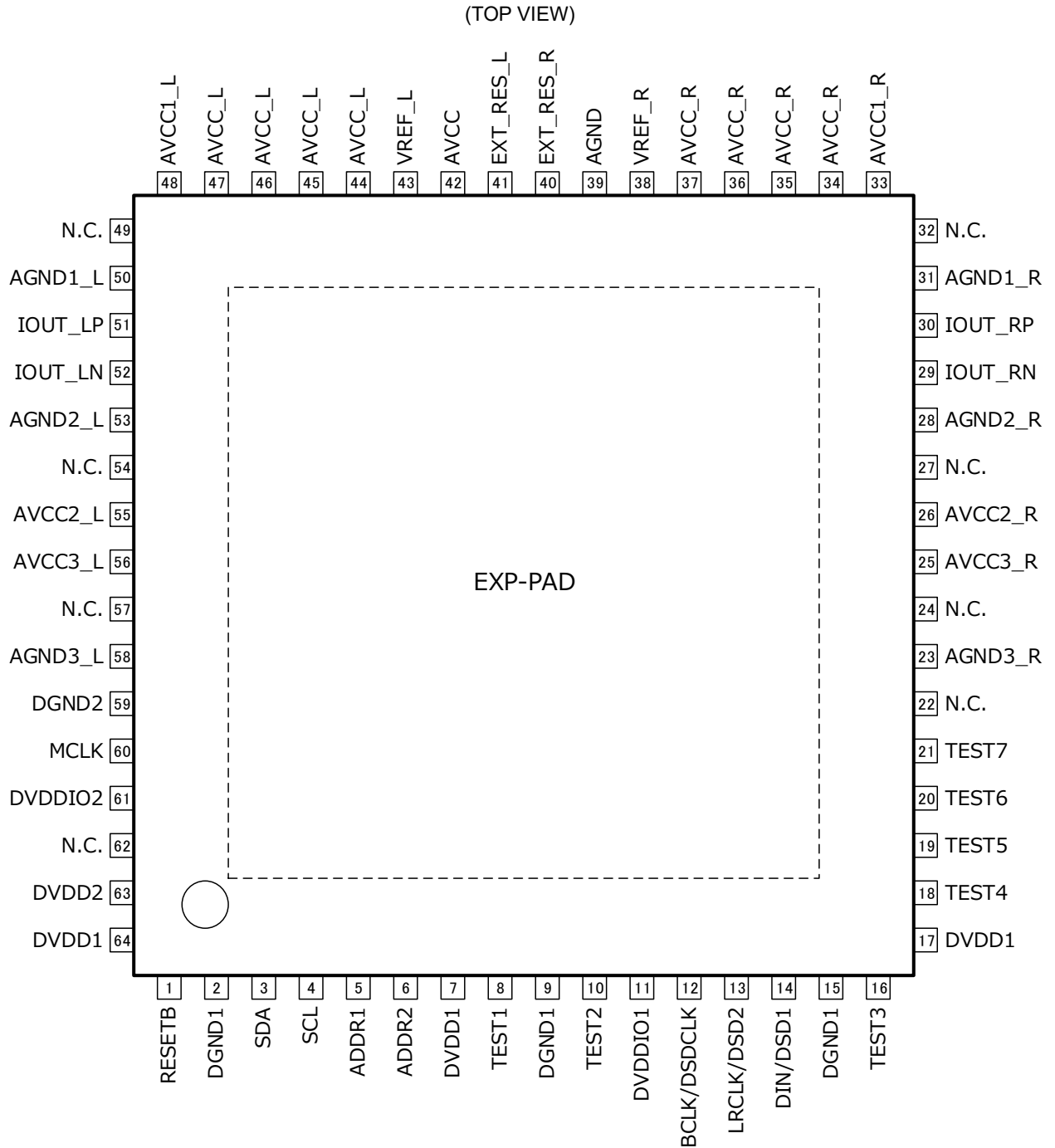
Figure 2. Pin Configuration
