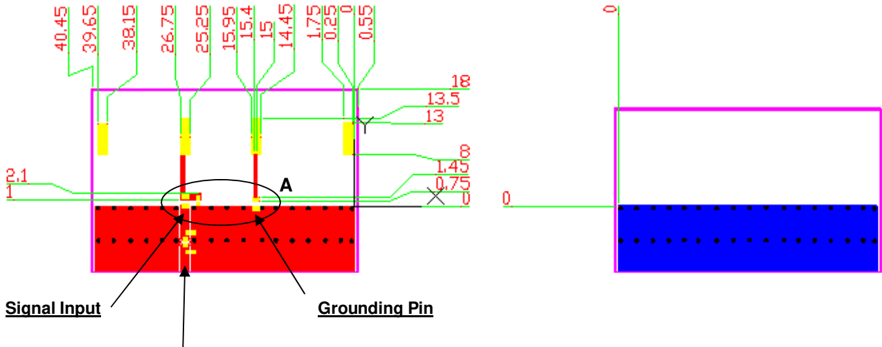
Transmission Line with 50Ω Impedance Characteristic
