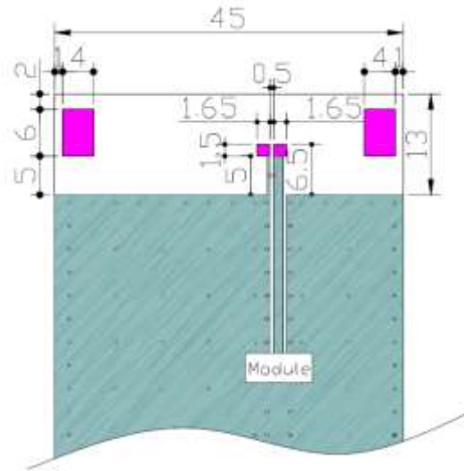
Layout dimensions of the PA.700.J Antenna.
