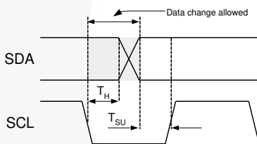
Figure 45. Data Transfer Timing
