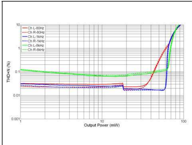
Figure 14. THD+N vs. output power - R_L = 16 \Omega , out-of-phase, V_{CC} = 3.6 V
