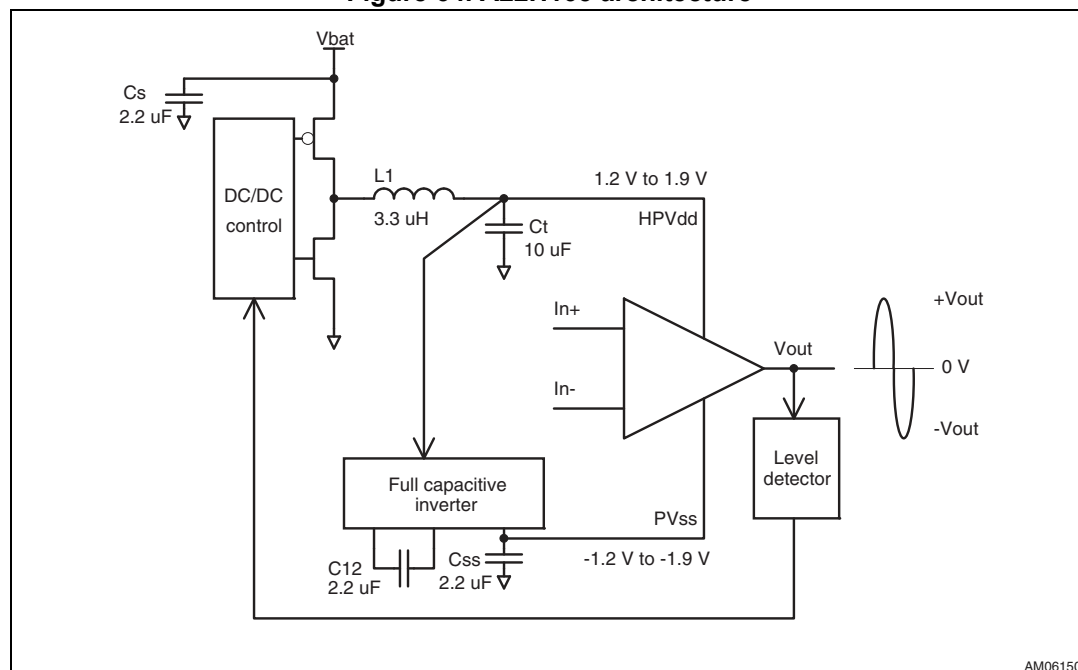
Figure 64. A22H165 architecture
