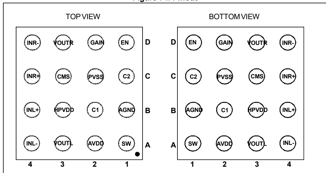
Figure 74. Pinout
