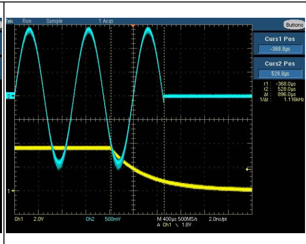
Figure 63. Shutdown
