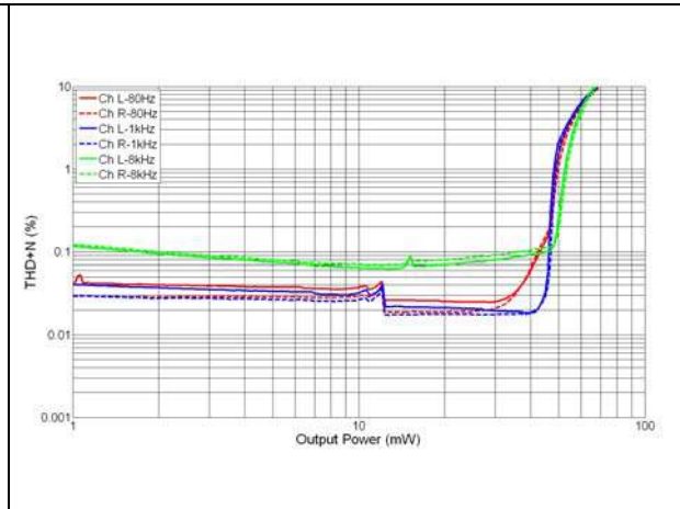
Figure 15. THD+N vs. output power - R_L = 16 \Omega , in-phase, V_{CC} = 4.8 V
