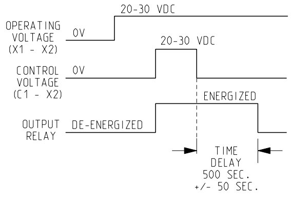
TIMING DIAGRAM
