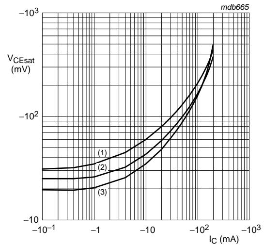
I_C/I_B = 10 (1) T_{amb} = 150^\circ\text{C} (2) T_{amb} = 25^\circ\text{C} (3) T_{amb} = -55^\circ\text{C}
