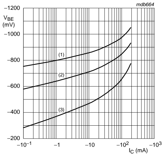
V_{CE} = -6\text{ V} (1) T_{amb} = -55^\circ\text{C} (2) T_{amb} = 25^\circ\text{C} (3) T_{amb} = 150^\circ\text{C}
