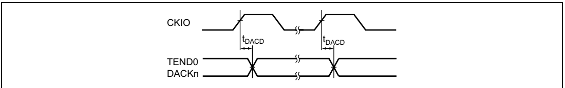
Figure 25.44 DACK, TEND Output Timing
