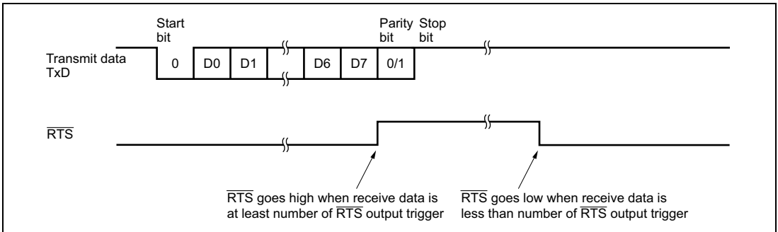
Figure 16.11 \overline{\text{RTS}} Control Operation
