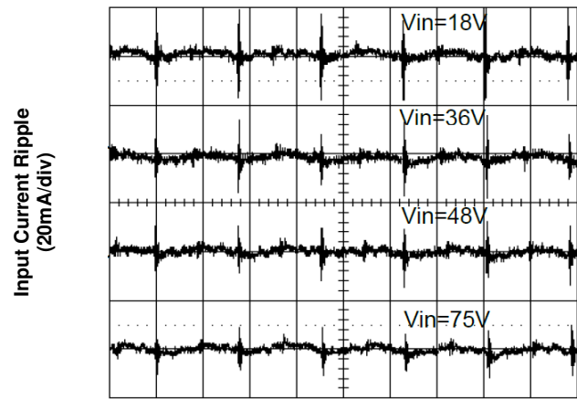
Figure 6. Input Reflected Ripple Current at Full Load
