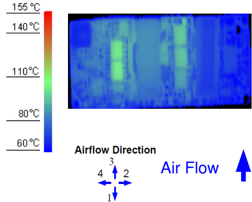
Figure 10. Thermal Image for Airflow Direction 3 (7.4A output, 55°C ambient, 200 LFM, typical Vin open frame unit)
