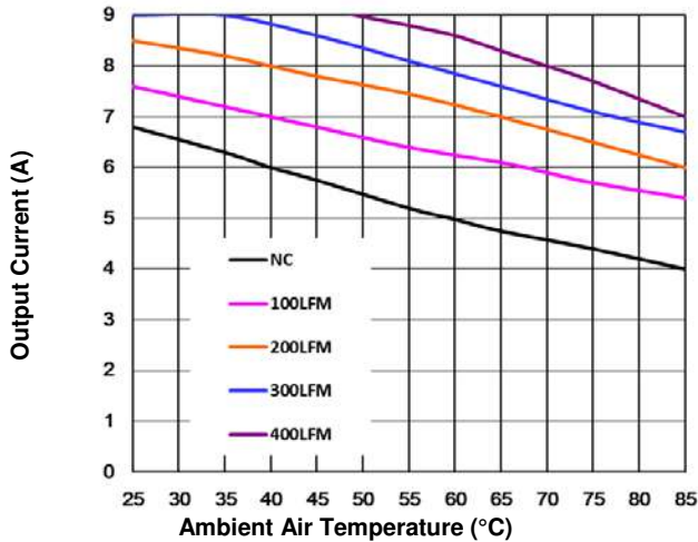
Figure 9. Current Derating Curve for Airflow Direction 3 (Ref. Fig. 10 for Airflow Direction; Vin = 36V, open frame unit using solder interface)
