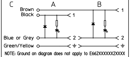
ELECTRICAL DIAGRAM E66XXXXXXA1X
