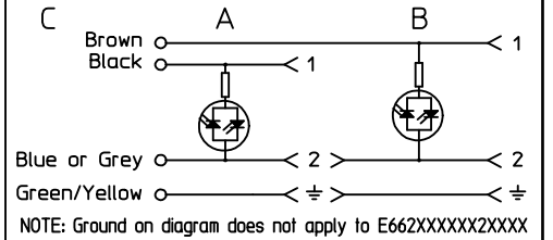
ELECTRICAL DIAGRAM E66XXXXXXC4X
