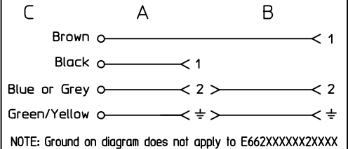
ELECTRICAL DIAGRAM E66XXXXXX000
