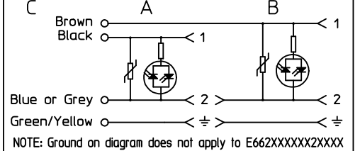
ELECTRICAL DIAGRAM E66XXXXXXS0X
