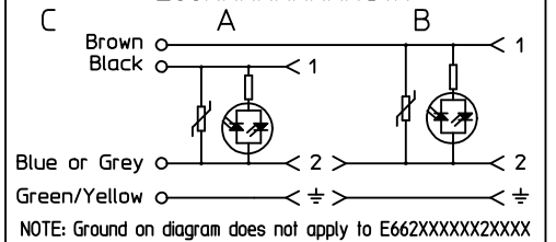
ELECTRICAL DIAGRAM E66XXXXXXS0X
