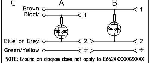
ELECTRICAL DIAGRAM E66XXXXXXC4X
