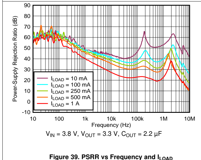
Figure 39. PSRR vs Frequency and I_{LOAD}
