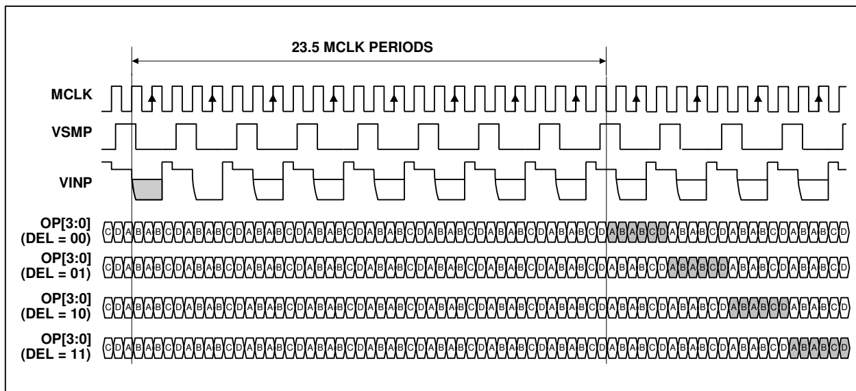
Figure 19 Mode 2 Operation
