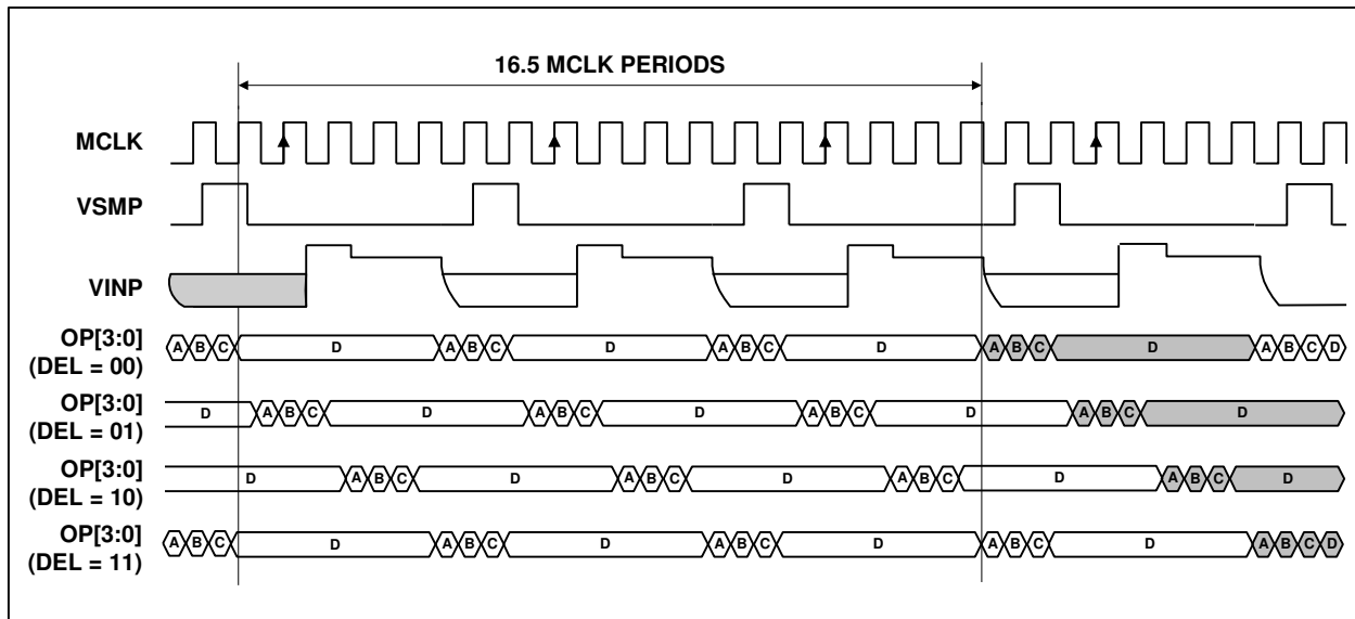
Figure 18 Mode 1 Operation
