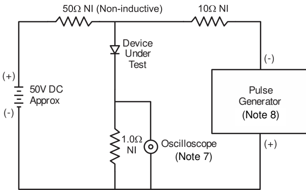
Figure 5 Reverse Recovery Time Characteristic and Test Circuit
