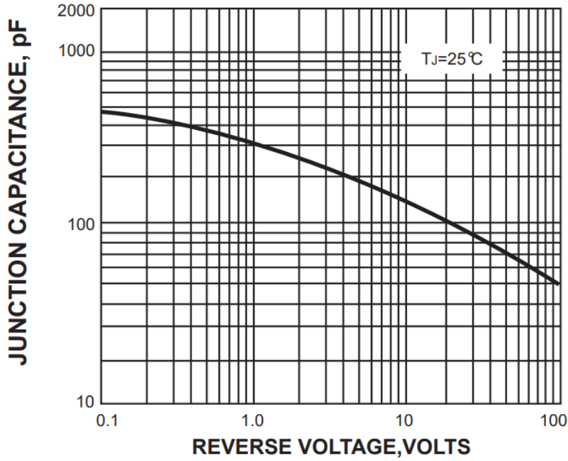
FIG. 5-TYPICAL JUNCTION CAPACITANCE
