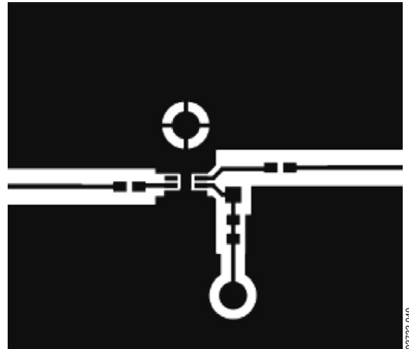
Figure 43. Component Side
