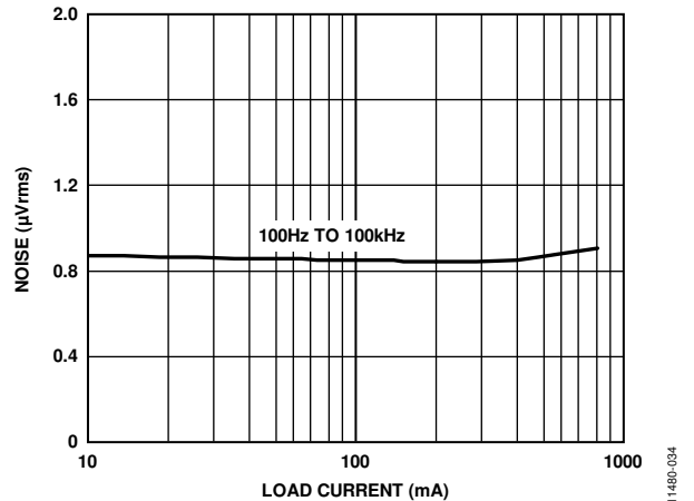
Figure 34. RMS Output Noise vs. Load Current ( I_{LOAD} ), 100 Hz to 100 kHz, ADM7151-02, V_{OUT} = 4V
