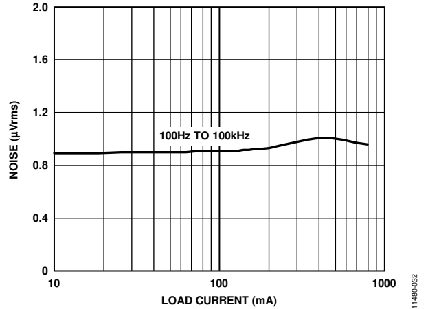
Figure 32. RMS Output Noise vs. Load Current ( I_{LOAD} ), 100 Hz to 100 kHz, ADM7151-04, V_{OUT} = 5V
