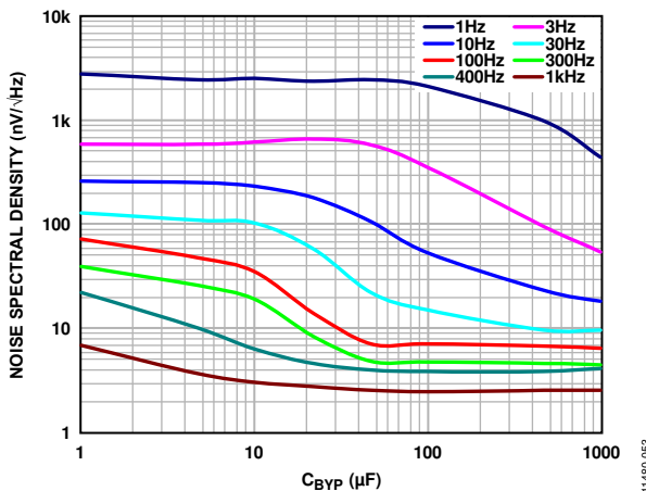
Figure 53. Noise Spectral Density vs. C BYP for Different Frequencies
