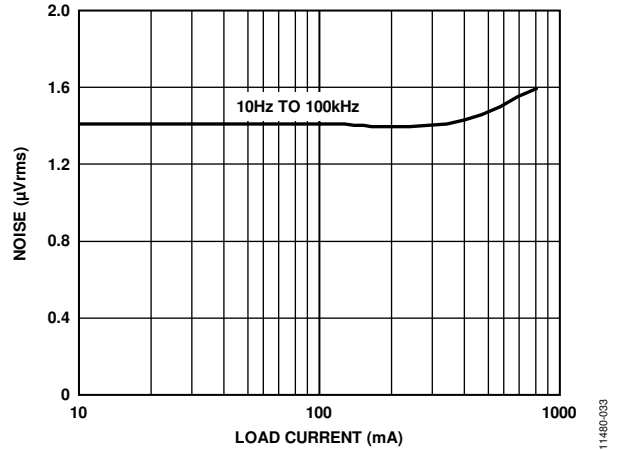
Figure 33. RMS Output Noise vs. Load Current ( I_{LOAD} ), 10 Hz to 100 kHz, ADM7151-02, V_{OUT} = 4V
