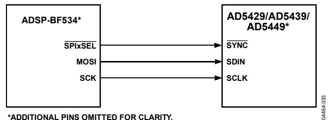
Figure 49. ADSP-BF534-to-AD5429/AD5439/AD5449 Interface
