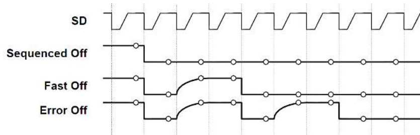
Figure 35. OK Severity Encoding Waveforms
