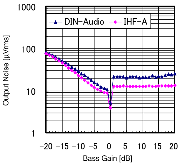
Figure 11. Output Noise vs Bass Gain
