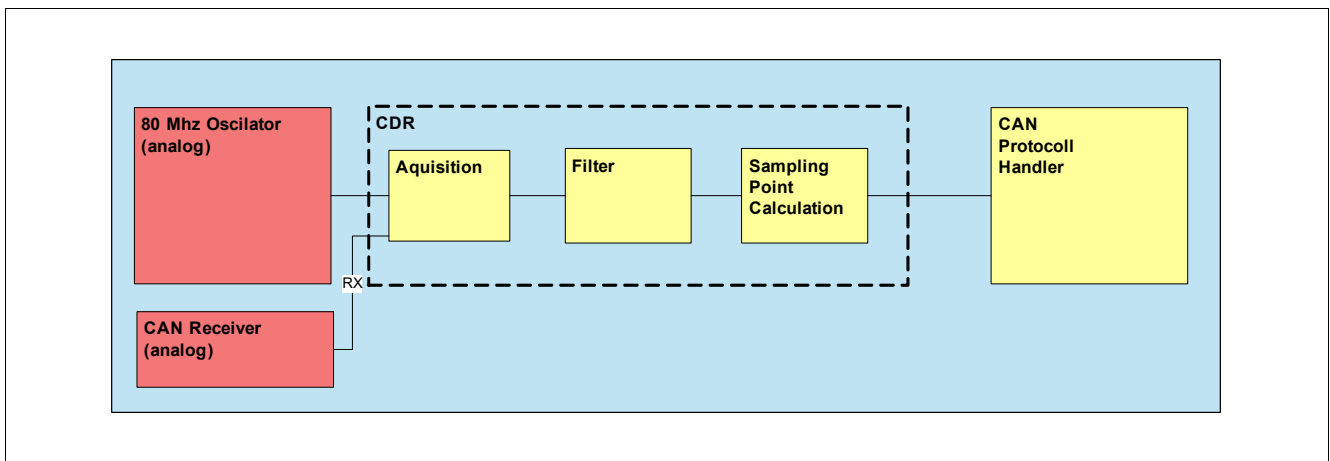
Figure 26 Clock and Data Recovery Block Diagram
