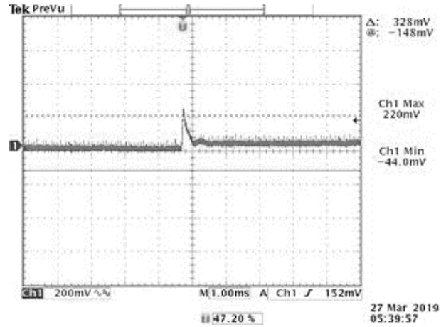
Figure 13. 50%-75% Load Transients at V_{in} = 54 V @ T_a = 25^{\circ}C Figure 14. 75%-50% Load Transients at V_{in} = 54 V @ T_a = 25^{\circ}C
