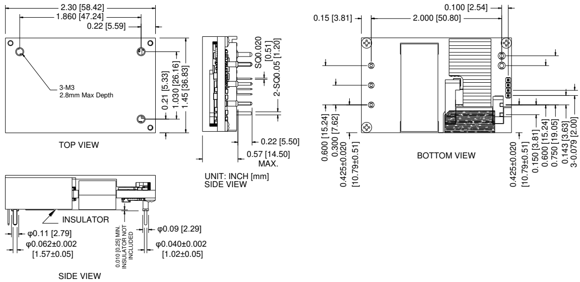
Figure 32. ORQP-X5M12AG outline
