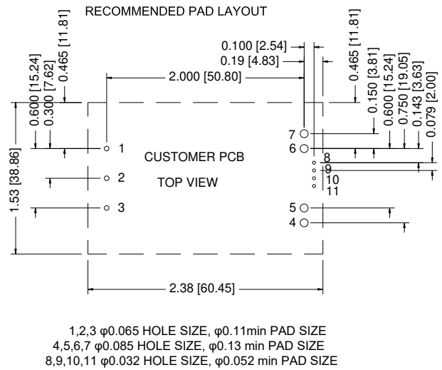
Figure 34. Recommended Pad Layout-2
