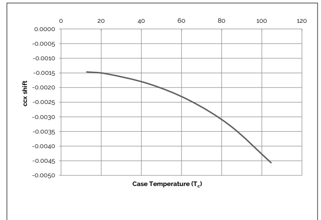
Figure 16: Typical ccx Shift vs. Case Temperature
