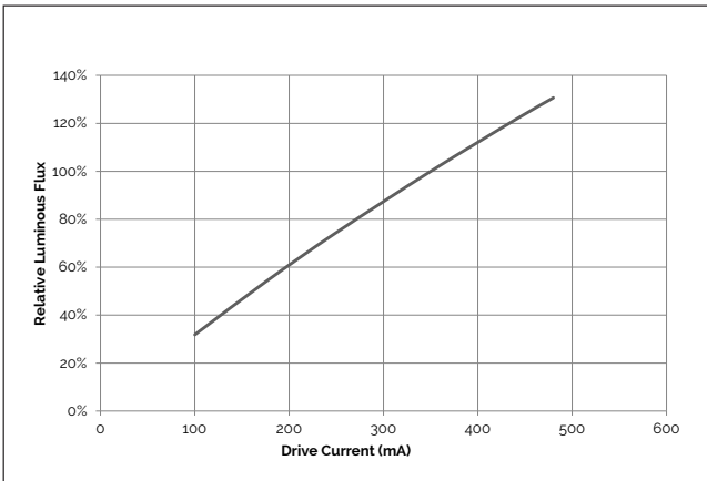
Figure 13: Typical Relative Flux vs. Current V6B HD 1,2
