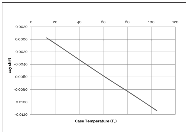
Figure 17: Typical ccy Shift vs. Case Temperature
