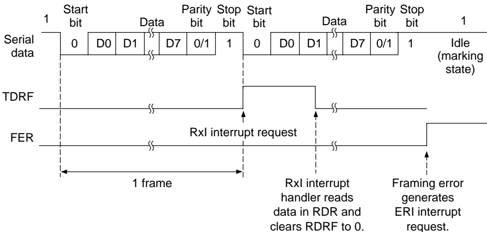
Figure 14.9 SCI Receive Operation
