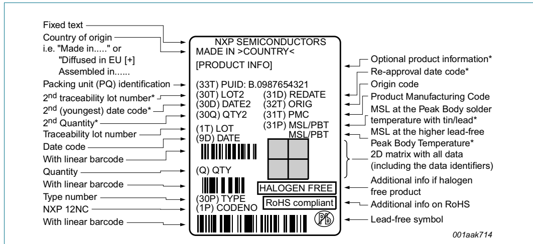
Fig 24. Example of typical box and reel information barcode label
