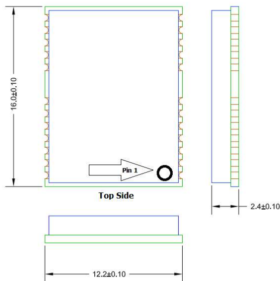
Package Outline Drawing
