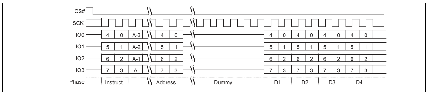
Figure 68 Read Any Register, QPI Mode, command sequence [50]
