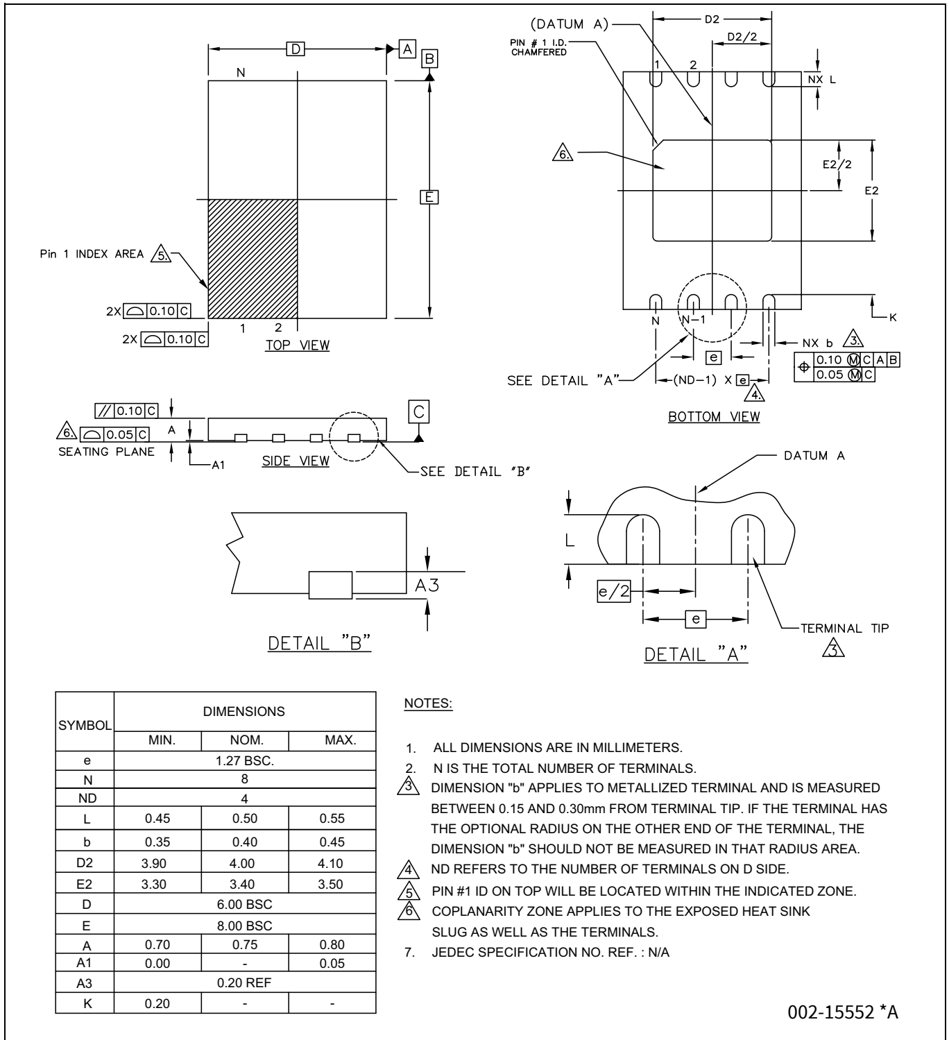
Figure 118 WSON 8-Lead DFN 6.0 × 8.0 × 0.8 mm (WNH008) WNH008 4.0 × 3.4 mm E-Pad (SAWN)
