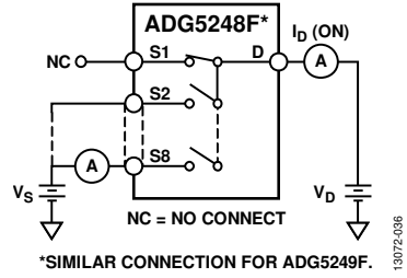
Figure 37. On Leakage
