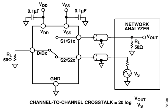
Figure 40. Channel-to-Channel Crosstalk
