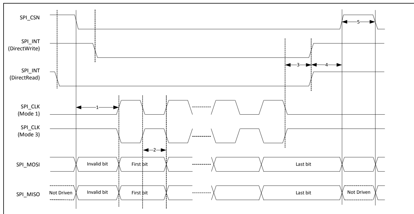
Figure 21. SPI Timing, Mode 1 and 3
