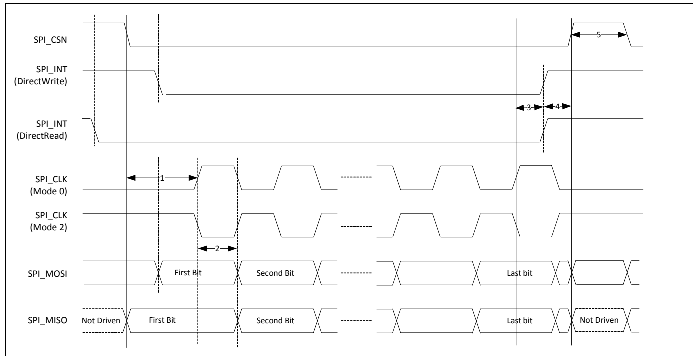
Figure 20. SPI Timing, Mode 0 and 2
