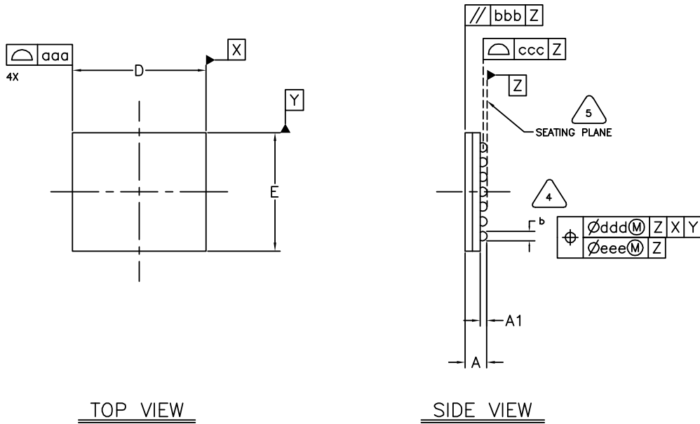
Figure 22. 49-Ball FcBGA Mechanical Drawing
