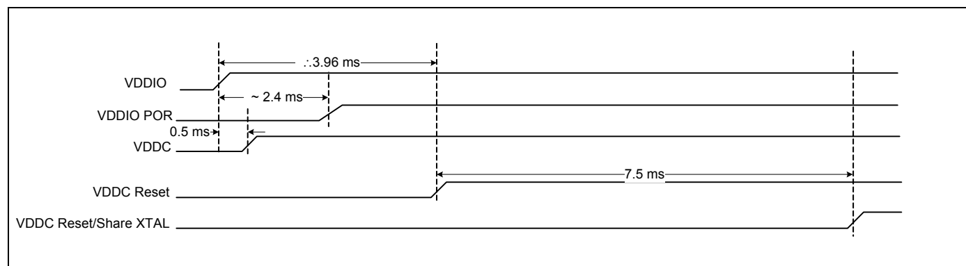
Figure 8. Startup Timing
