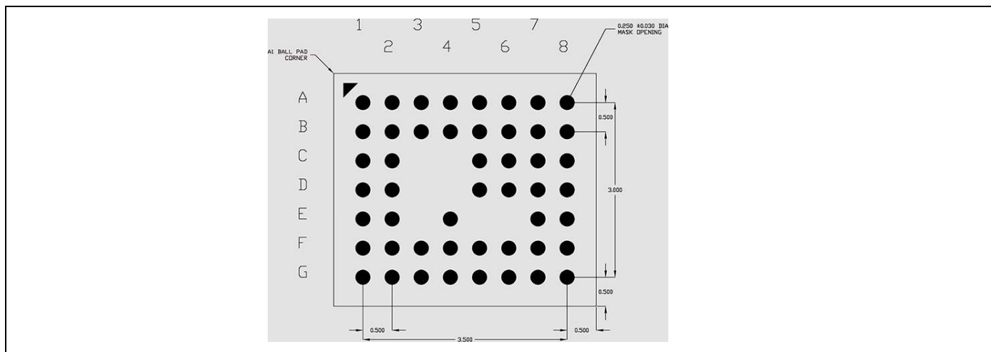
Figure 7. Ball-Out for the 49-Ball FcBGA
