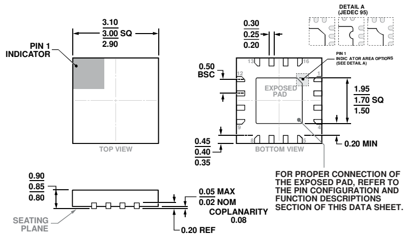
Figure 22. 16-Lead Lead Frame Chip Scale Package [LFCSP] 3 mm × 3 mm Body and 0.85 mm Package Height (HCP-16-1) Dimensions shown in millimeters
