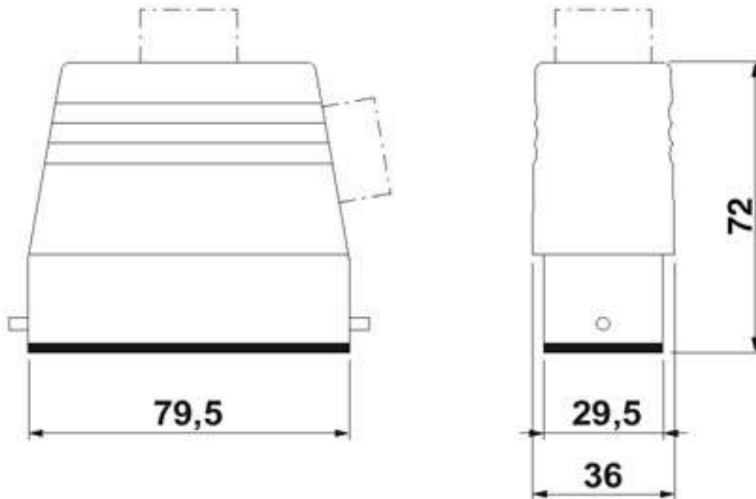
Dimensioned drawing
